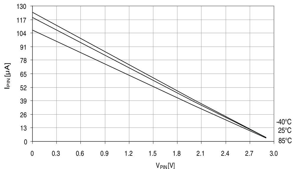
Figure 38-21. I/O pin pull-up resistor current vs. input voltage. V_{CC} = 3.0V .
