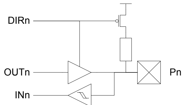
Figure 16-3. I/O configuration - Totem-pole with pull-up (on input).
