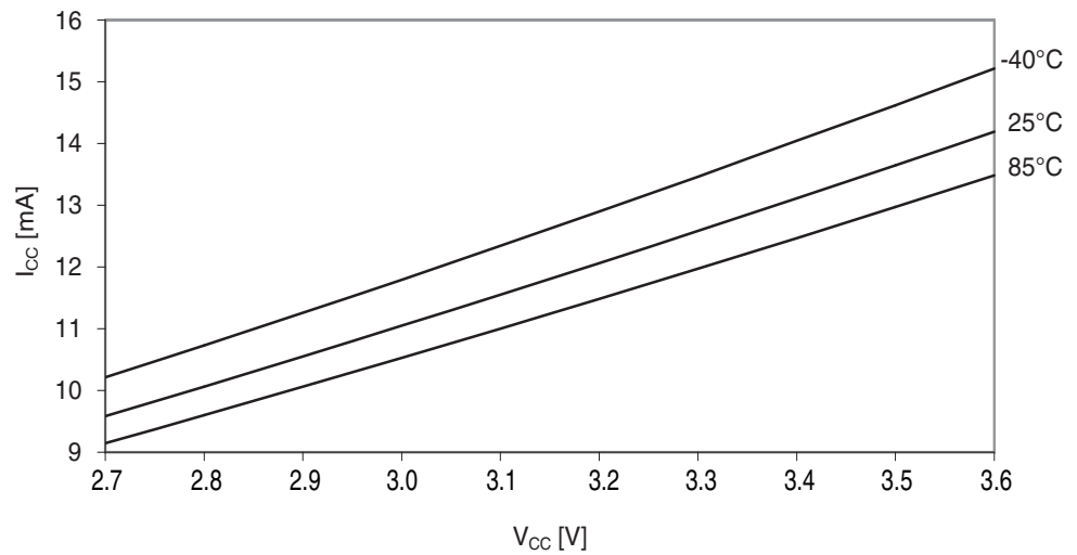
Figure 38-7. Active mode supply current vs. V_{CC} .
