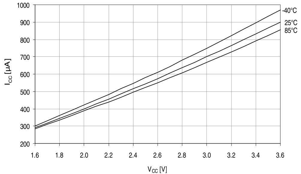
Figure 38-4. Active mode supply current vs. V_{CC} .
