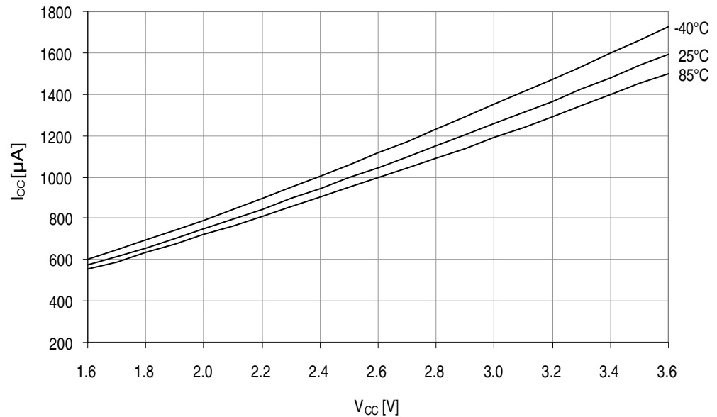
Figure 38-5. Active mode supply current vs. V_{CC} .
