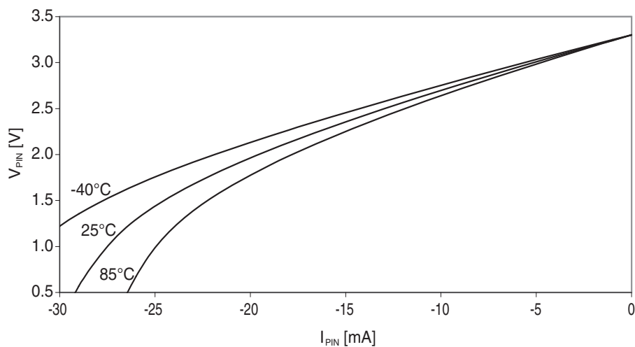
Figure 38-25. I/O pin output voltage vs. source current. V_{CC} = 3.3V .
