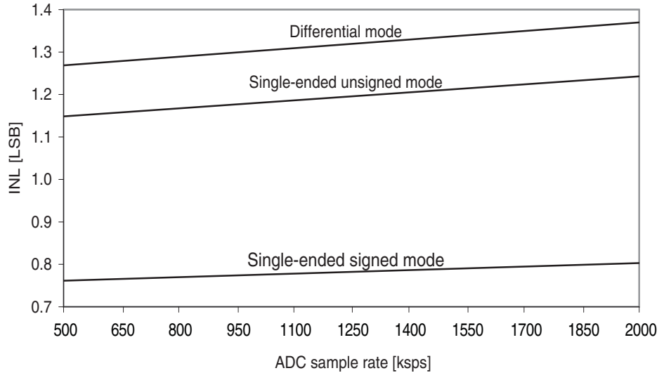
Figure 38-36. INL error vs. sample rate. T = 25^{\circ}\text{C} , V_{CC} = 3.6\text{V} , V_{REF} = 3.0\text{V} external.
