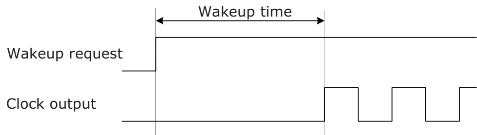
Figure 37-2. Wake-up time definition.
