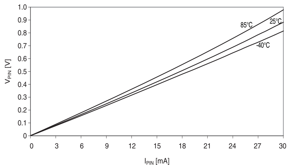
Figure 38-28. I/O pin output voltage vs. sink current. V_{CC} = 3.0V .
