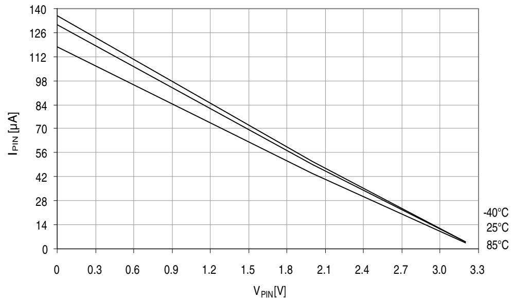
Figure 38-64. Reset pin pull-up resistor current vs. reset pin voltage. V_{CC} = 3.3V .
