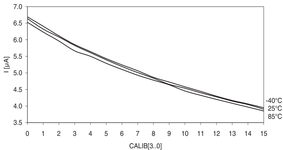
Figure 38-56. Analog comparator current source vs. calibration value. V CC = 3.0V.
