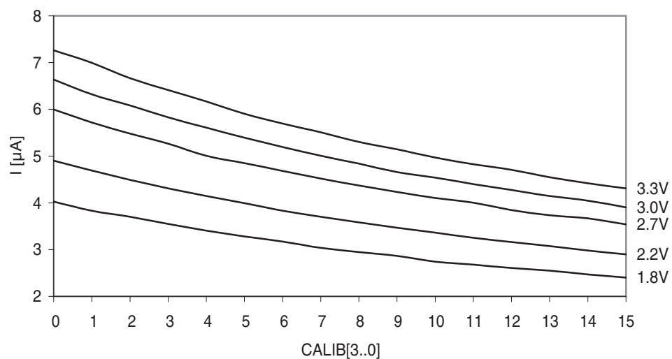
Figure 38-55. Analog comparator current source vs. calibration value. Temperature = 25°C.
