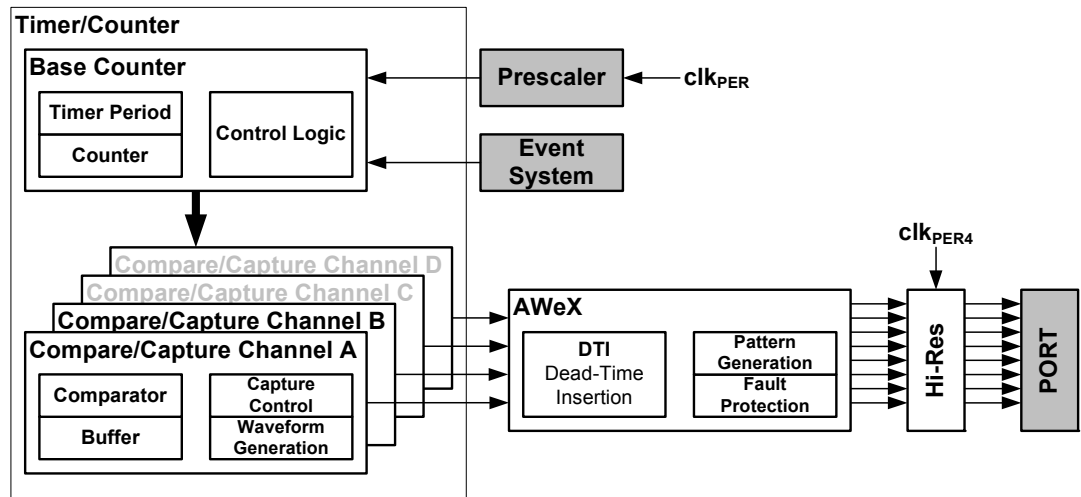
Figure 17-1. Overview of a Timer/Counter and closely related peripherals.
