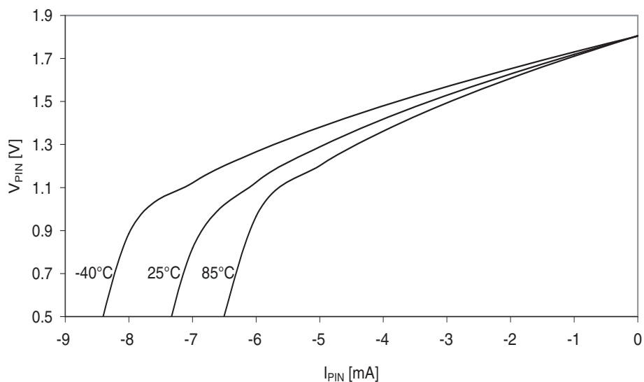
Figure 38-23. I/O pin output voltage vs. source current. V_{CC} = 1.8V .
