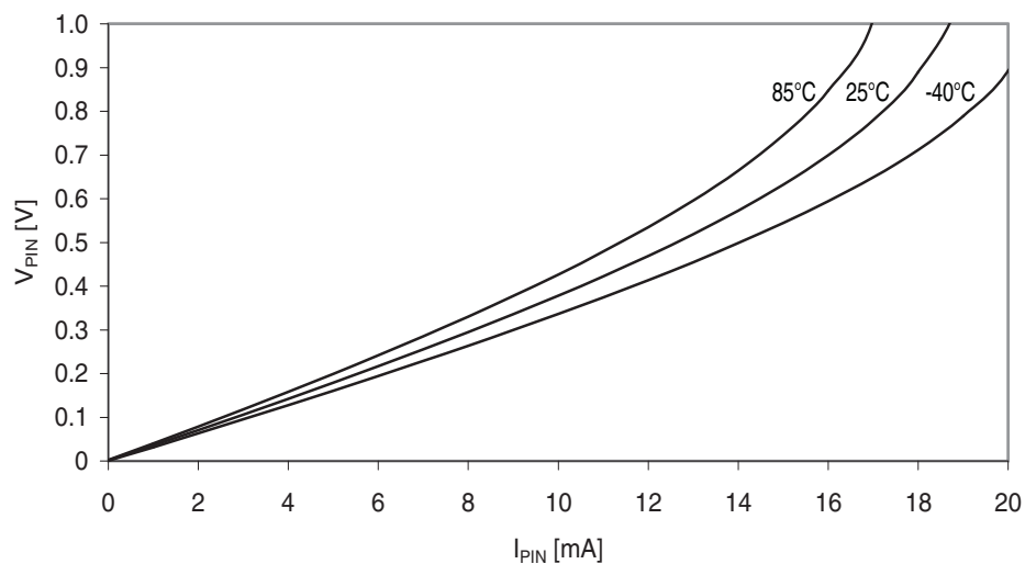
Figure 38-27. I/O pin output voltage vs. sink current. V_{CC} = 1.8V .
