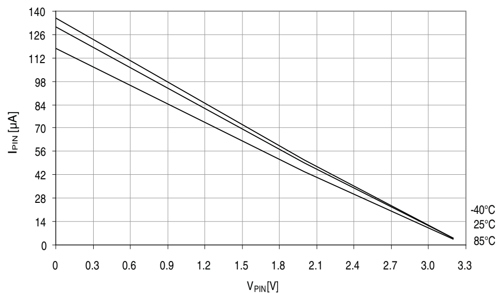
Figure 38-22. I/O pin pull-up resistor current vs. input voltage. V_{CC} = 3.3V .
