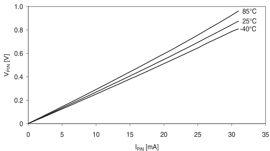
Figure 38-29. I/O pin output voltage vs. sink current. V_{CC} = 3.3V .
