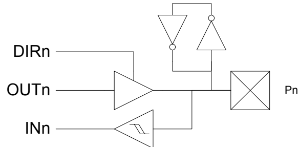
Figure 16-4. I/O configuration - Totem-pole with bus-keeper.
