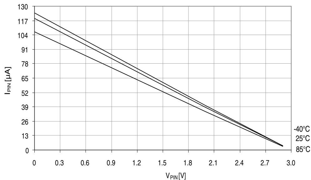
Figure 38-63. Reset pin pull-up resistor current vs. reset pin voltage. V_{CC} = 3.0V .
